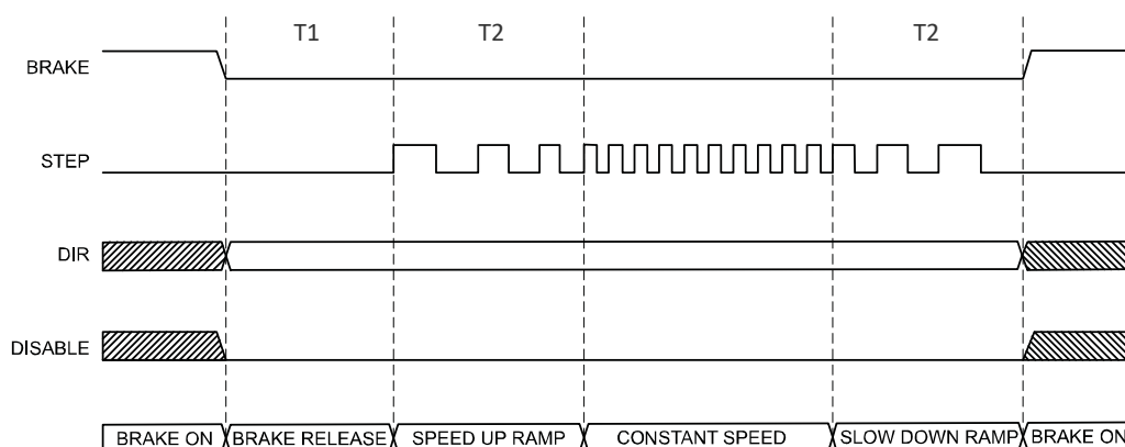
Figure 20: Axes I/O signals behavior
