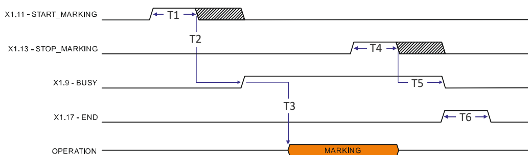
Figure 19: Marking process timing diagram
