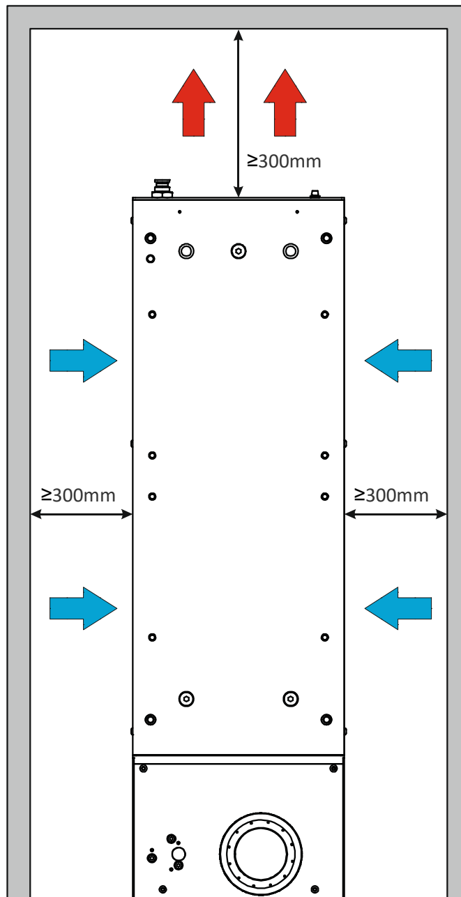
Figure 4: Installation environment
