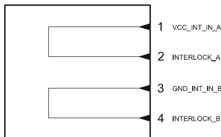
Figure 10: Interlock Muting Device electric diagram
