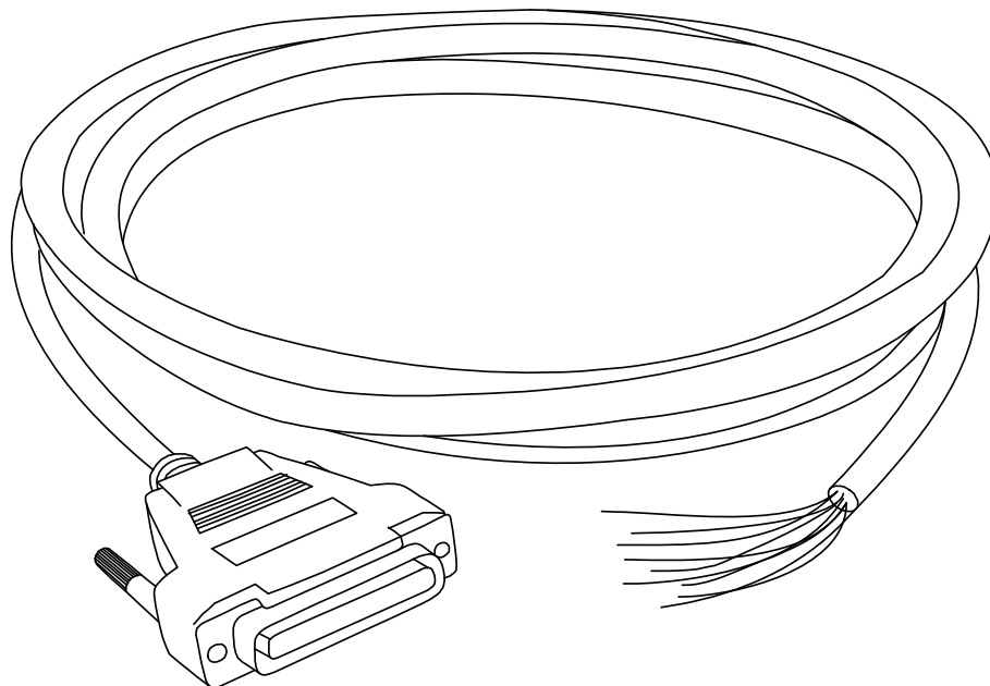
Figure 37: DB25-to-free leads cable (ordering no. 985350032)
