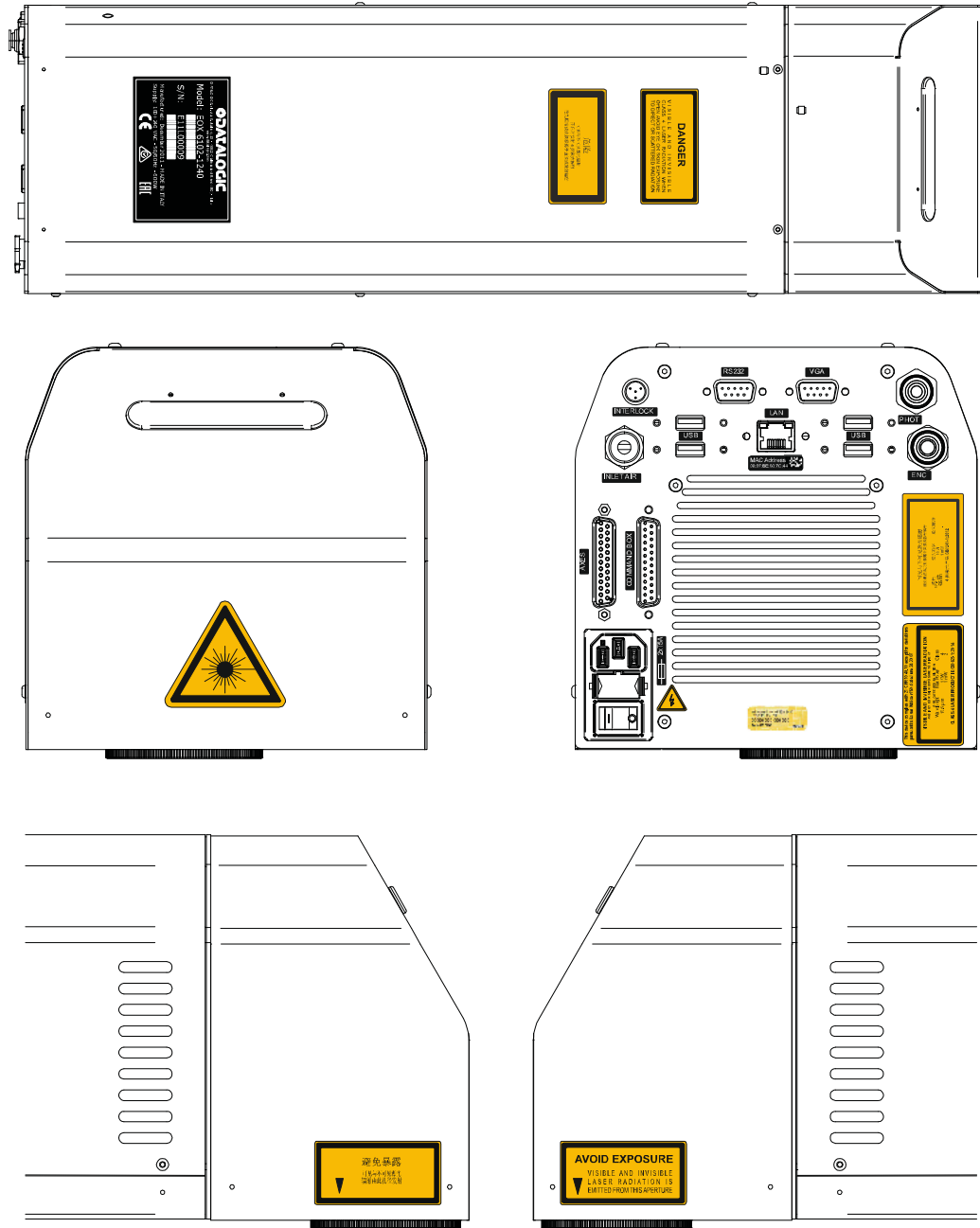
Figure 39: External labels location
