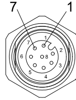
Figure 15: Encoder connector, female panel socket (front view)
