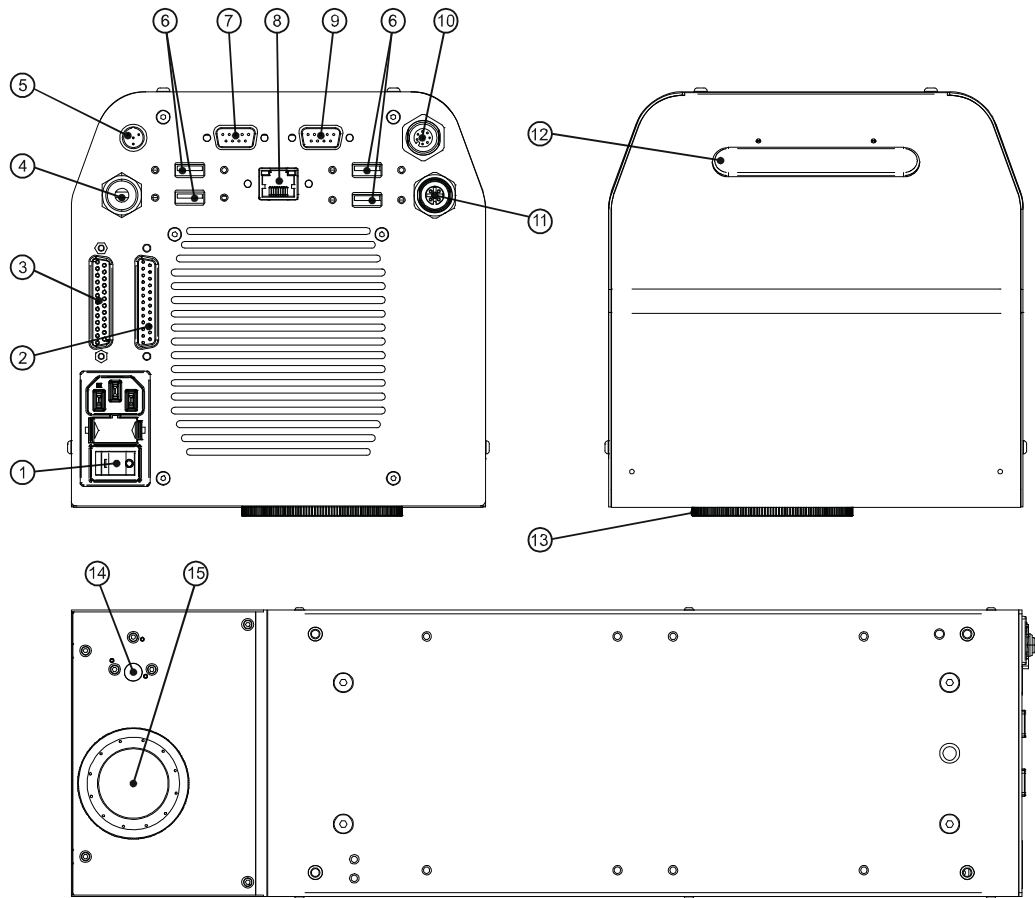
Figure 5: Laser marker overview
