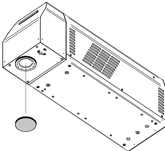
Figure 28: F-Theta scan lens protection cap removal
