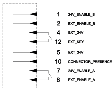
Figure 13: Command Box Muting Device electric diagram
