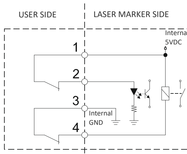
Figure 8: Interlock connector electric diagram
