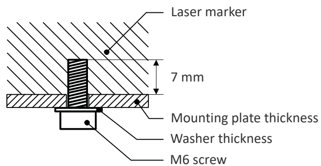
Figure 3: Length of mounting screws
