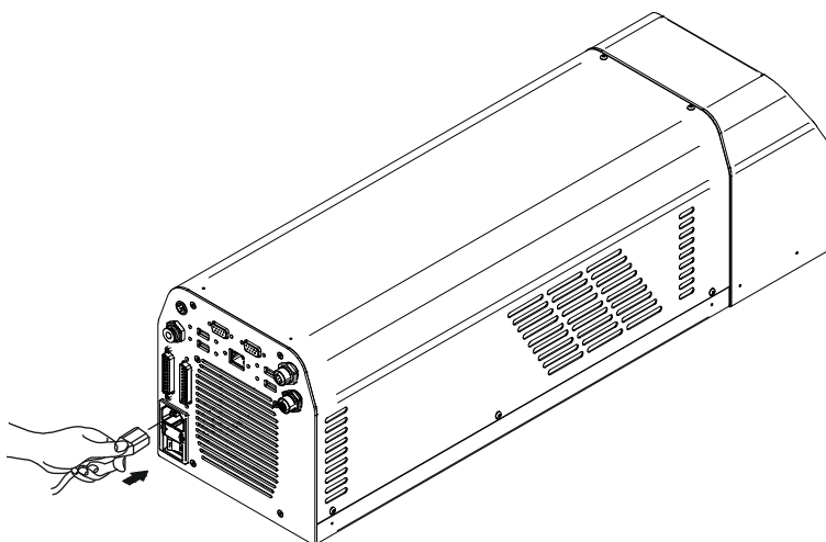
Figure 23: Connecting Power Supply cable
