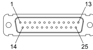
Figure 14: X2 - Axes connector, male panel plug (front view)
