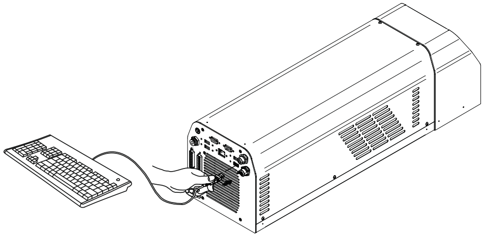
Figure 25: Connecting the keyboard
