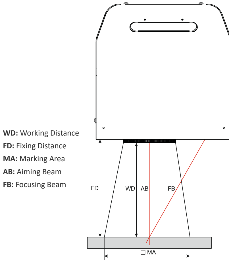
Figure 6: Marking Area
