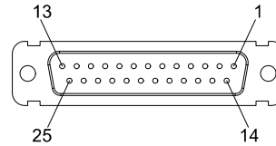
Figure 11: X1 - Command Box connector, female panel socket (front view)
