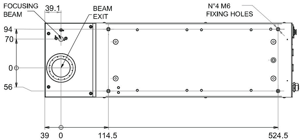
Figure 2: Fixing points
