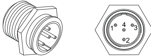
Figure 7: Male panel plug cod. TB4M (front view)
