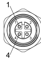
Figure 16: Photocell connector, female panel socket (front view)
